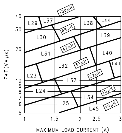
FIGURE 6. LM2673-ADJ
