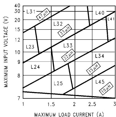
FIGURE 4. LM2673-5.0
