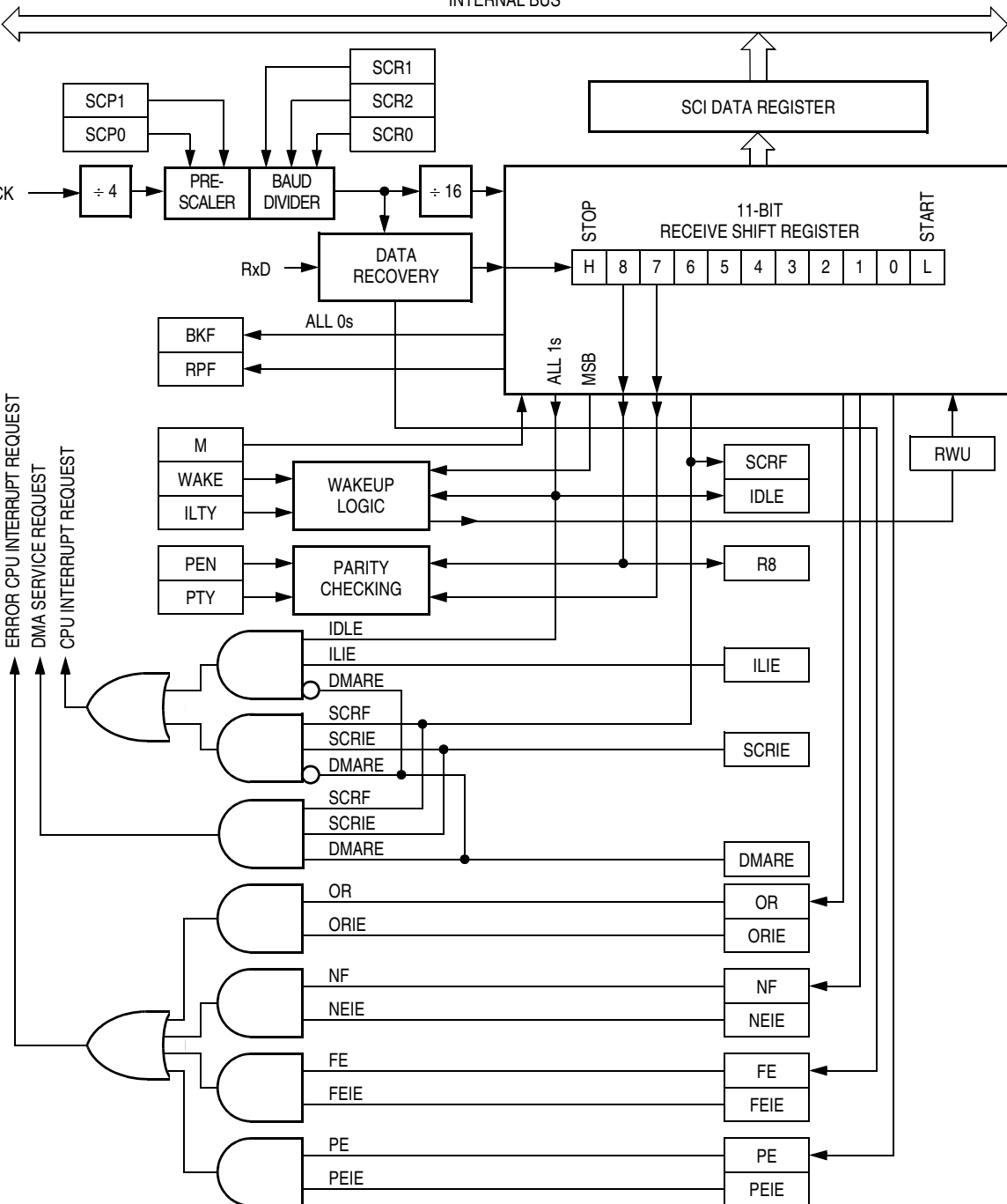
Figure 9-5. SCI Receiver Block Diagram
