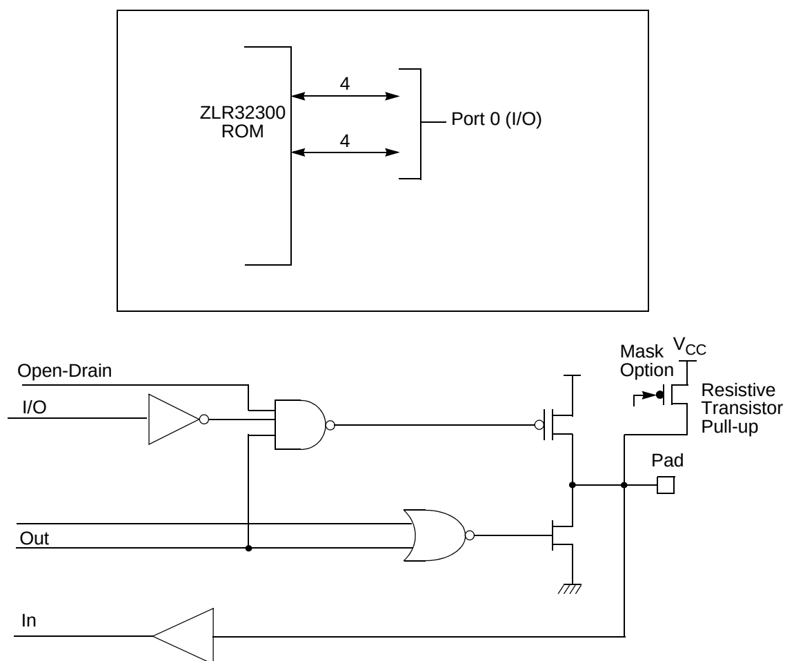
Figure 6. Port 0 Configuration
