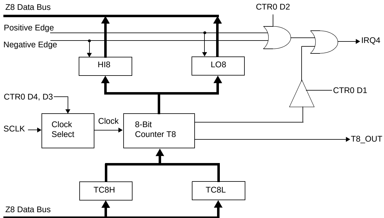
Figure 17.8-Bit Counter/Timer Circuits
