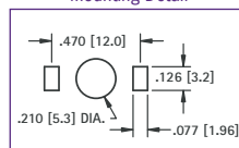
Mounting Detail
