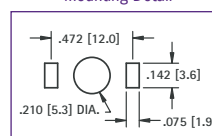
Mounting Detail
