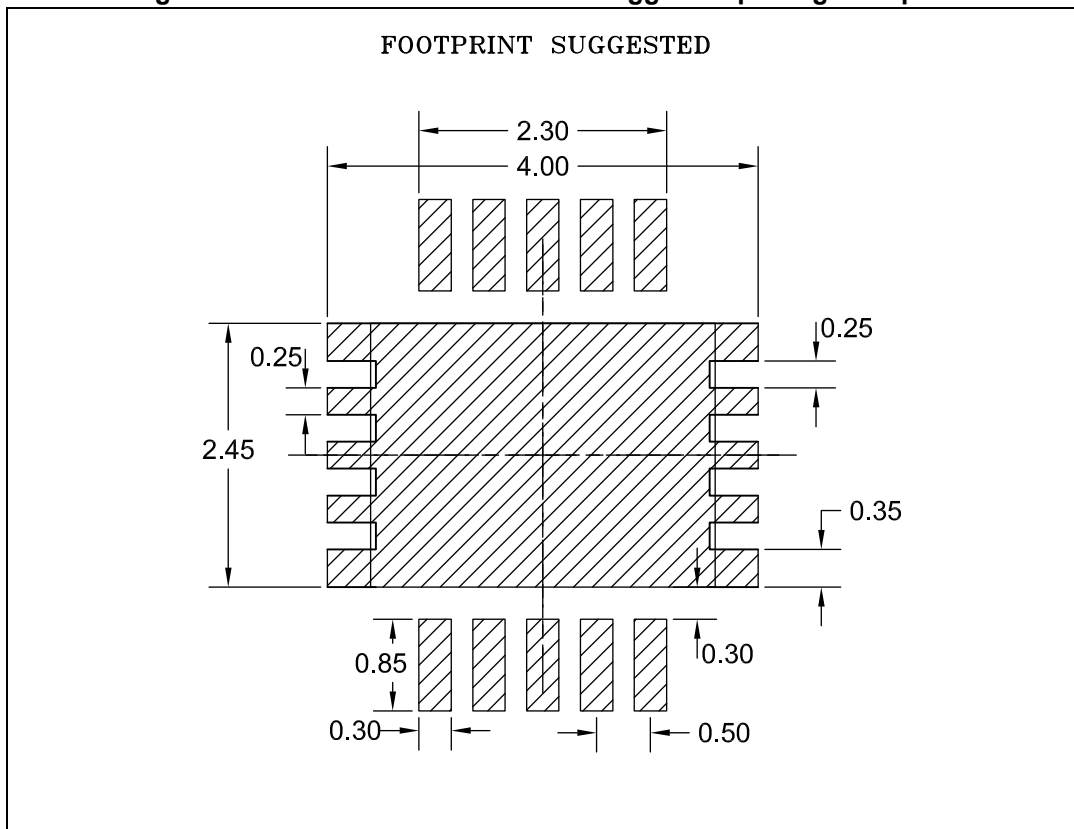
Figure 45. VFDFPN10 4 x 4 x 1.0 mm suggested package footprint
