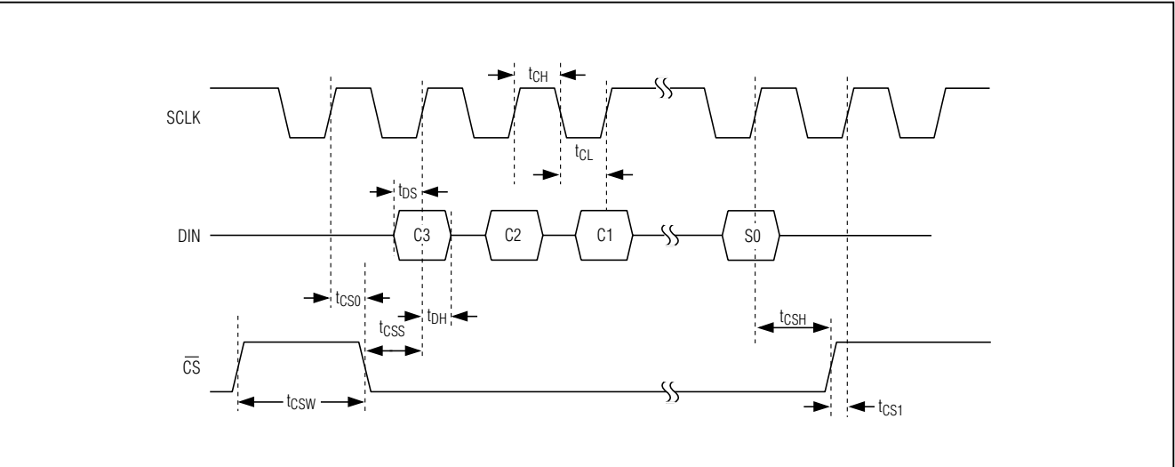
Figure 1. Timing Diagram
