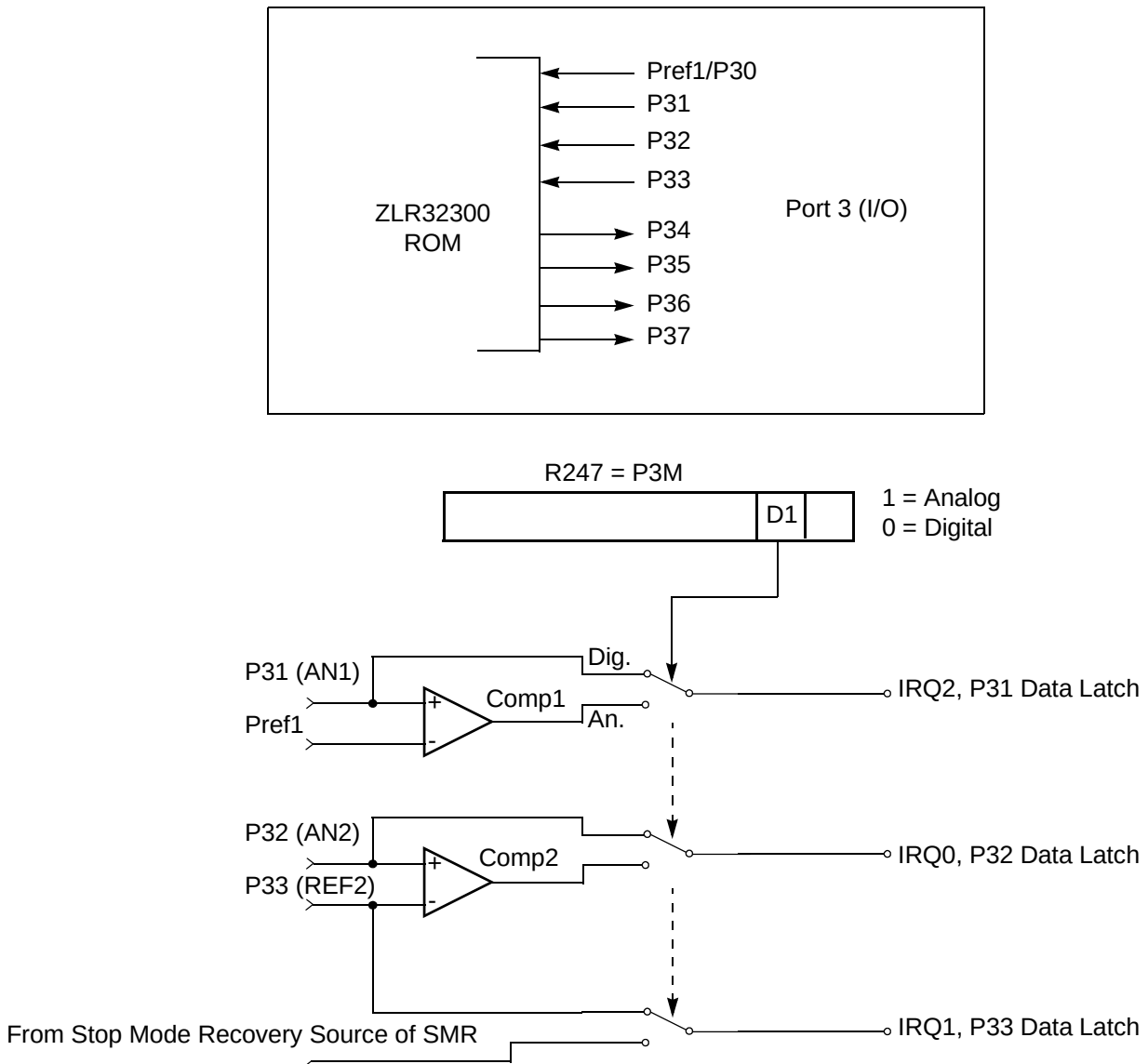
Figure 9. Port 3 Configuration
