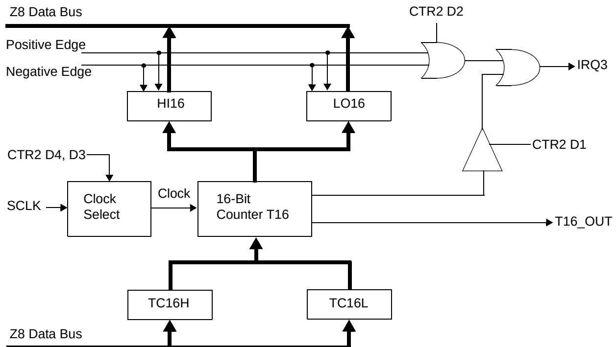
Figure 22.16-Bit Counter/Timer Circuits
