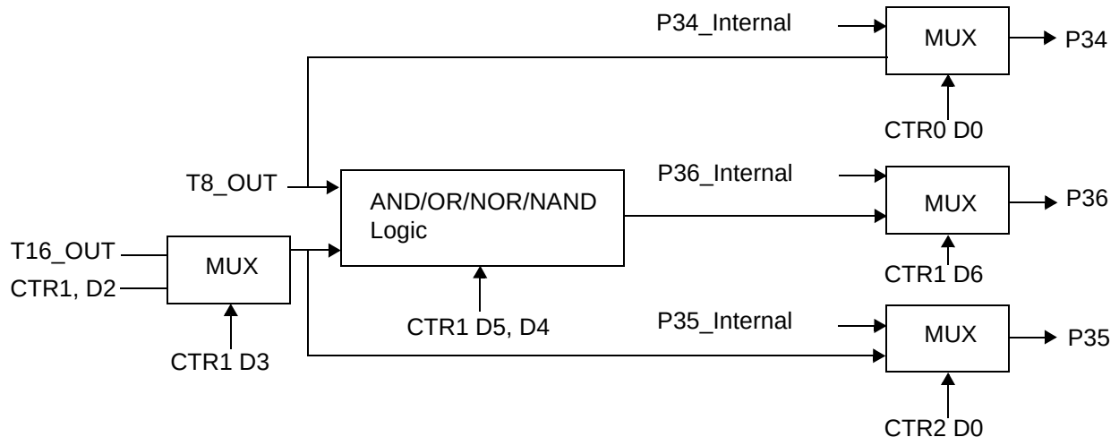
Figure 26. Output Circuit
