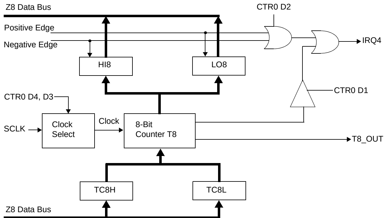
Figure 17.8-Bit Counter/Timer Circuits
