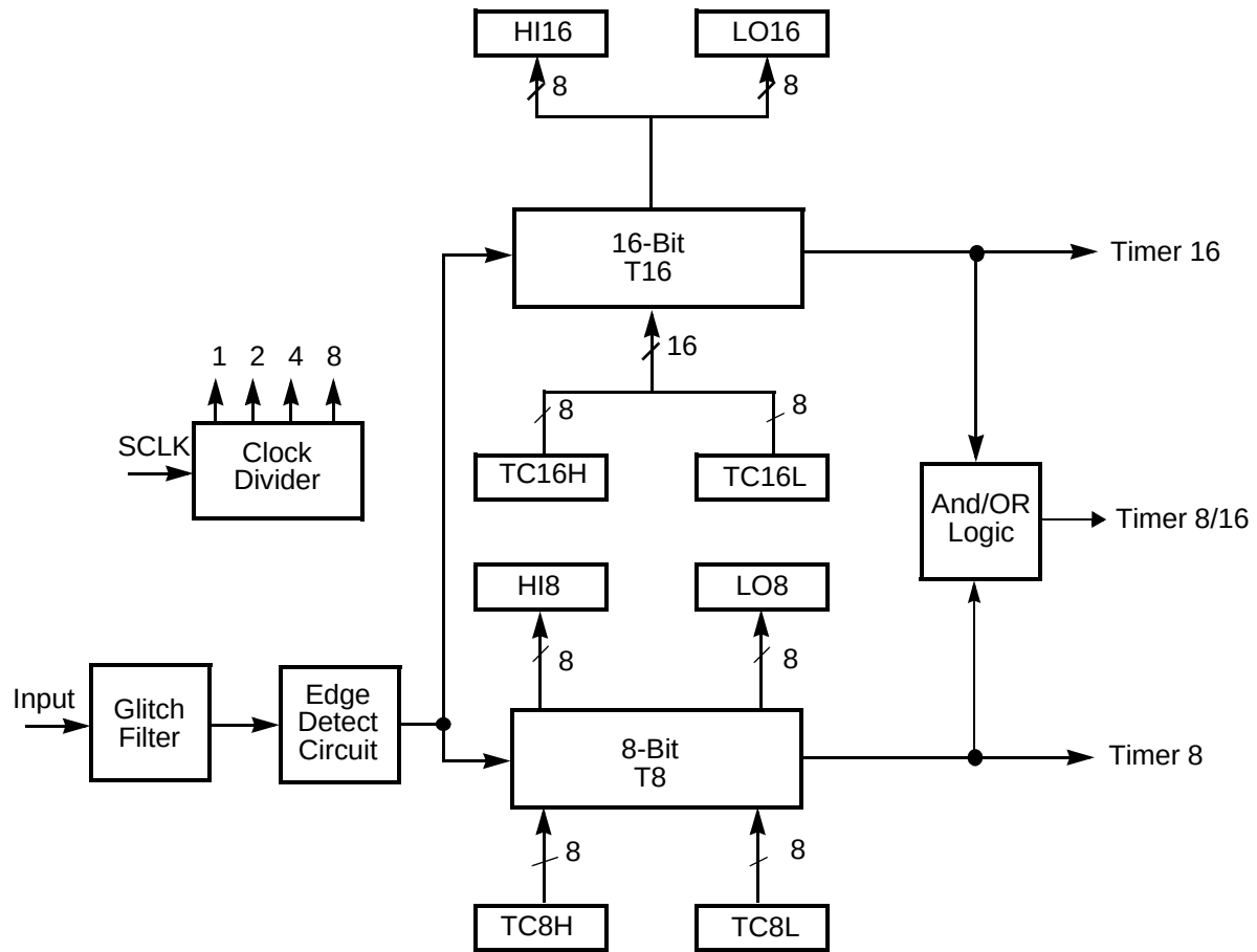
Figure 2. Counter/Timers Diagram
