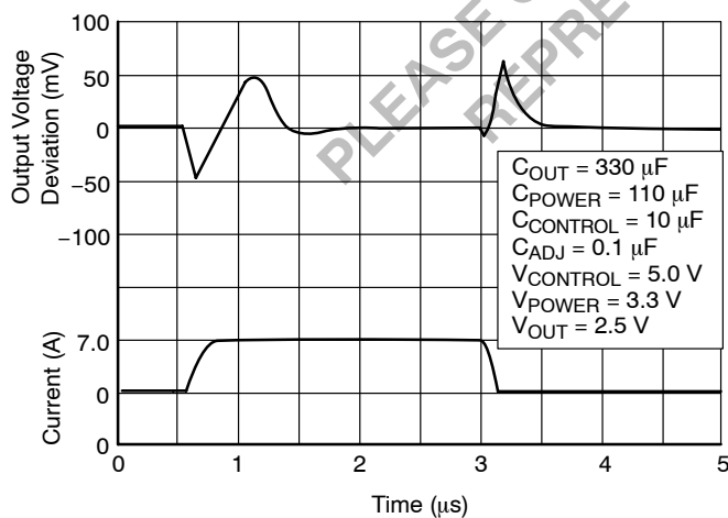
Figure 5. Transient Response
