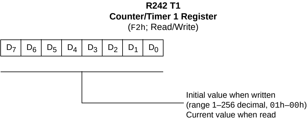
Figure 21. Counter/Timer 1 Register
