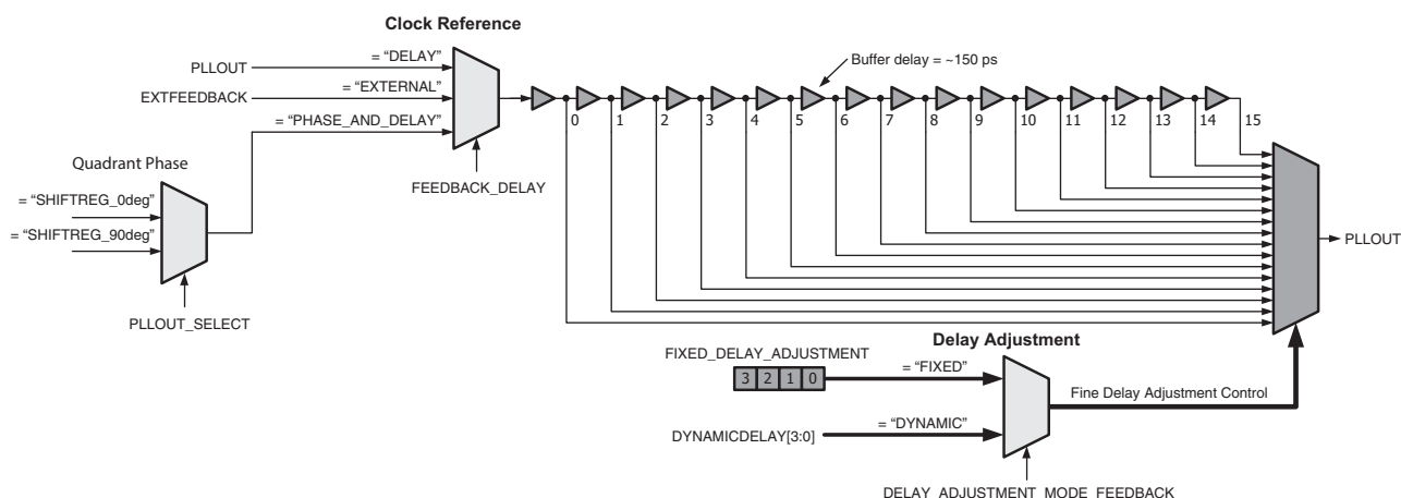
Figure 17-4. Fine Delay Adjust Control
