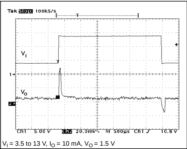
Figure 18. Line transient
