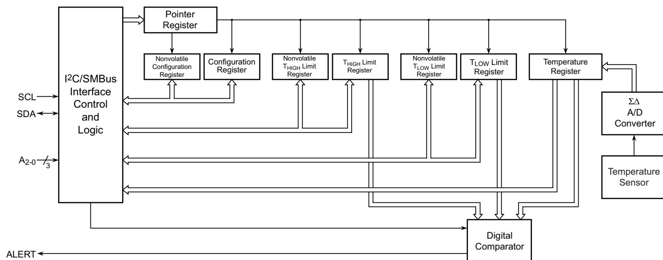
Figure 3-1. Block Diagram
