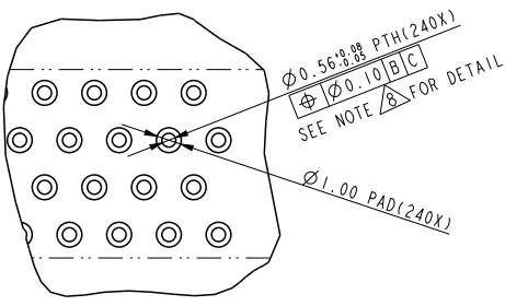
DETAIL D SCALE 3.000
