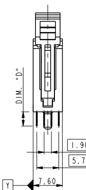
DETAIL A SCALE 3.000
