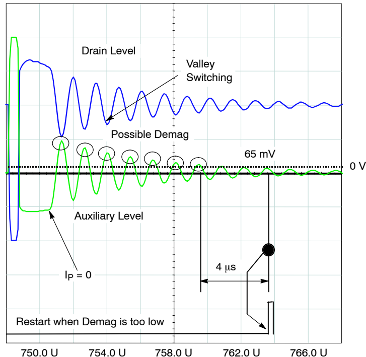
Figure 13. Core Reset Detection is done through an Auxiliary Winding Operated in Forward
