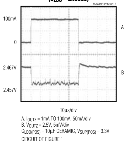
POSITIVE LINEAR REGULATOR LOAD TRANSIENT ( Q_{LDO} = 2N3905 )
