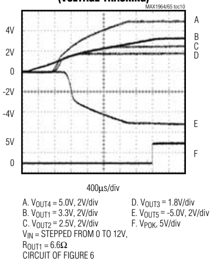
MAX1965 STARTUP WAVEFORM (VOLTAGE TRACKING)
