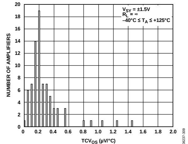
Figure 15. TCV_{OS} Distribution, SOT-23
