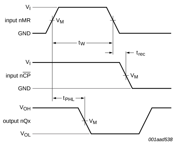
Fig 10. Propagation delays clock ( \overline{nCP} ) to output ( \overline{nQx} ), pulse width master reset ( \overline{nMR} ), and recovery time master reset ( \overline{nMR} ) to clock ( \overline{nCP} )
