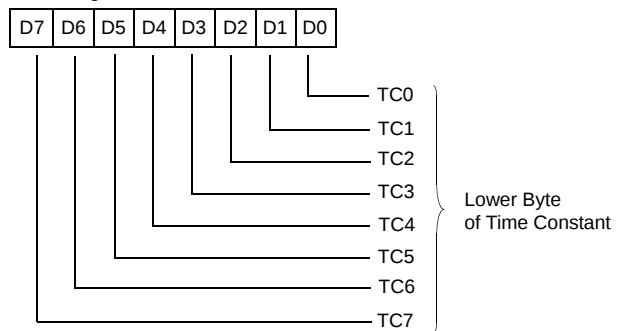
Read Register 12
