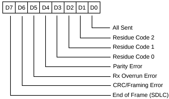
Read Register 1
