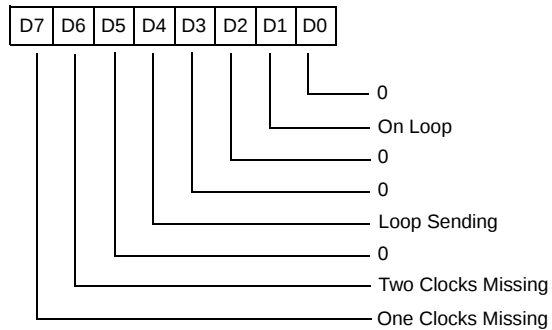
Read Register 10
