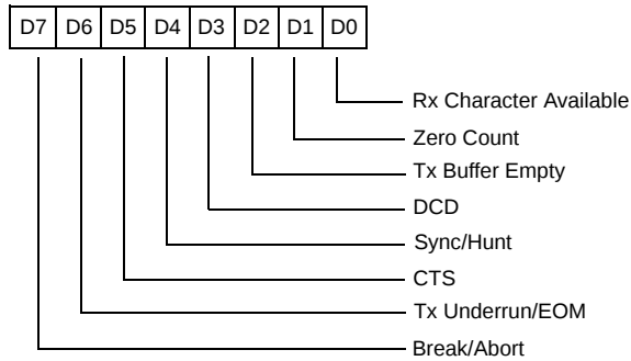
Read Register 0
