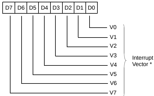
Read Register 2
