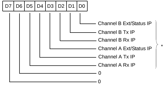
Read Register 3
