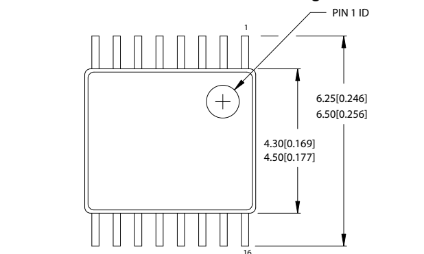
Figure 9. 16-Pin TSSOP 4.40 mm Body ZZ16
