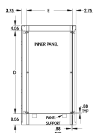
Rear View (Cross Section)
