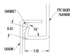
Rear View (Cross Section)
