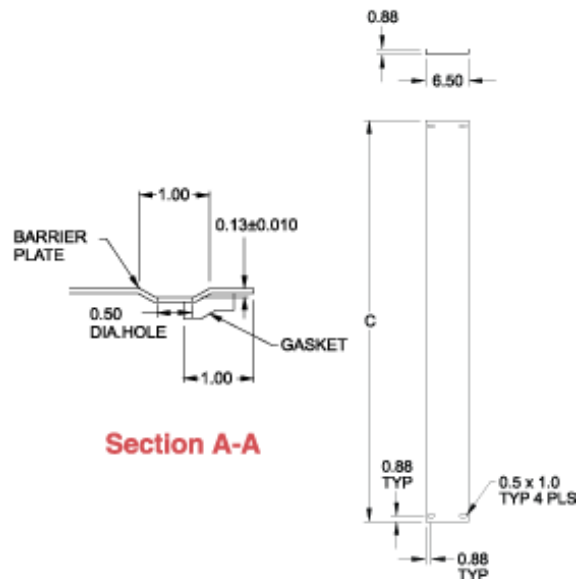
Panel Bridge Kit
