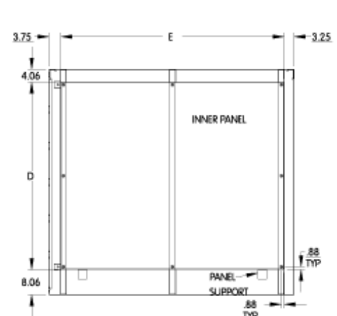
Rear View (Cross Section)
