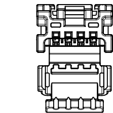
4 CIRCUIT RECEPTACLE WITHOUT LOCK BRIDGE POLARIZATION OPTION A
