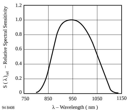
Figure 11. Relative Spectral Sensitivity vs. Wavelength
