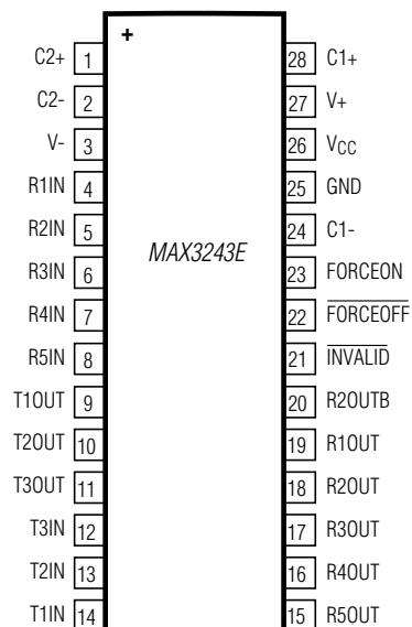
SO/SSOP/TSSOP
