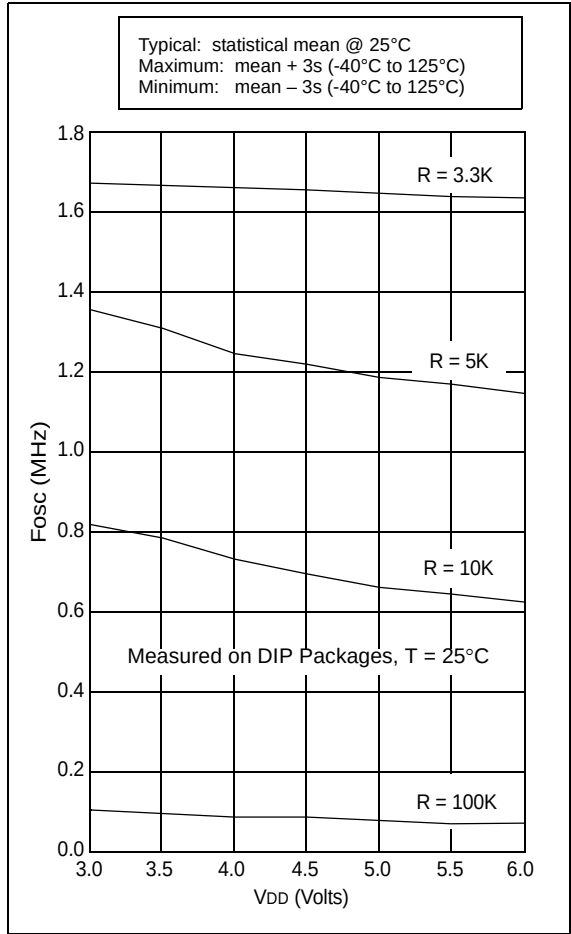
FIGURE 14-3: TYPICAL RC OSC FREQUENCY vs. V_{DD} , C_{EXT} = 100\text{ PF}
