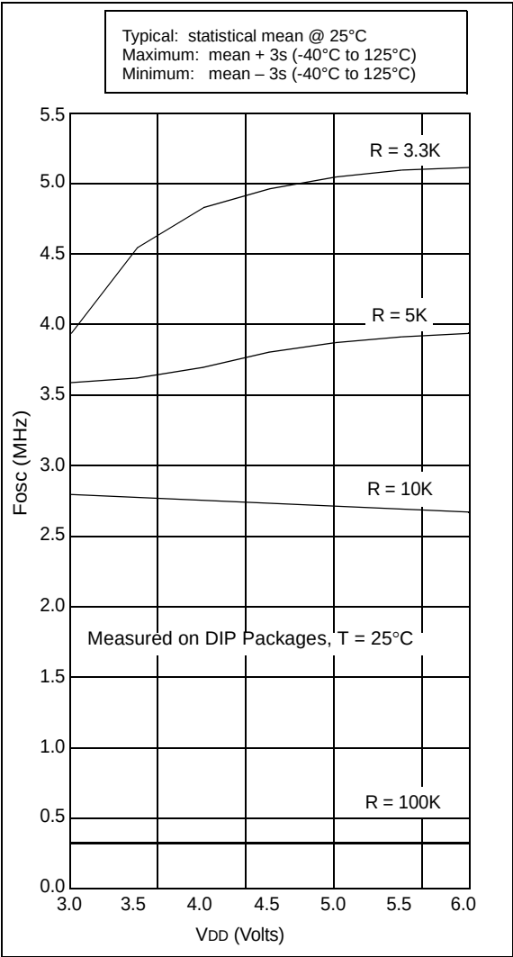
FIGURE 14-2: TYPICAL RC OSC FREQUENCY vs. V_{DD} , C_{EXT} = 20\text{ PF}
