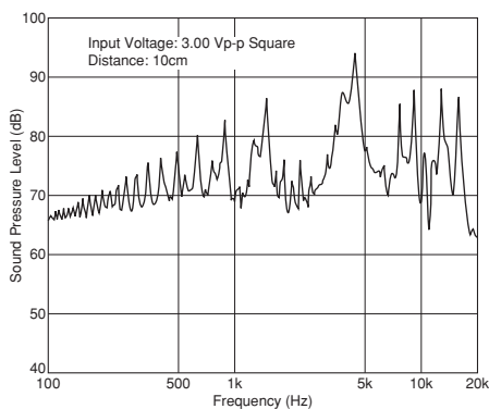
PKM22EPH4005-B0
