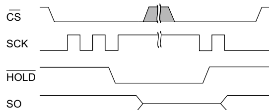
Figure 29. \overline{\text{HOLD}} Operation
