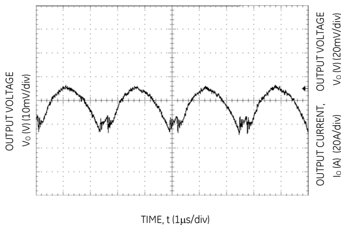
Figure 9. Typical output ripple and noise ( C_o = 6 \times 47 \mu F ceramic, V_{in} = 12V , I_o = I_{o,max} ).
