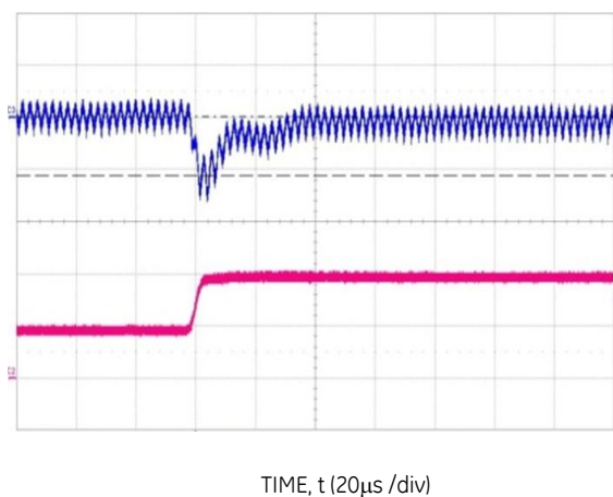
Figure 10. Transient Response to Dynamic Load Change from 50% to 100% at 12Vin, C_{out} = 6 \times 330 \mu F , C_{Tune} = 12nF & R_{Tune} = 200 \text{ ohms}
