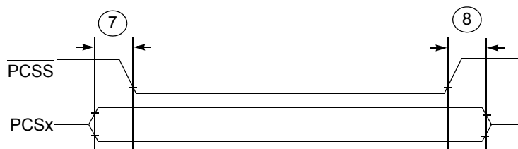
Figure 26. DSPI PCS Strobe (PCSS) Timing
