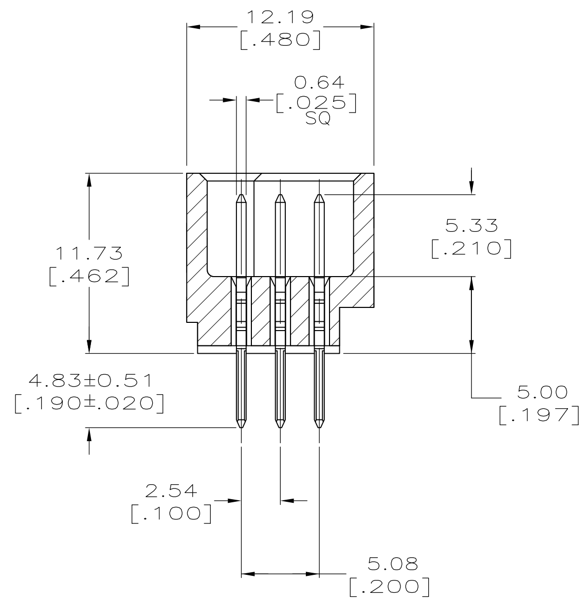
SECTION T-T
