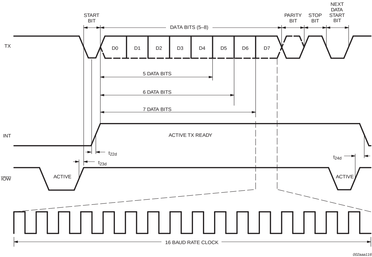
Fig 20. Transmit timing.
