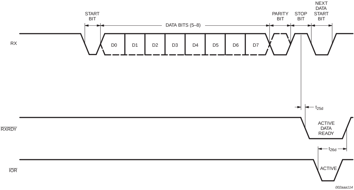
Fig 18. Receive ready timing in non-FIFO mode.
