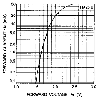
Fig. 8 Forward current vs. forward voltage
