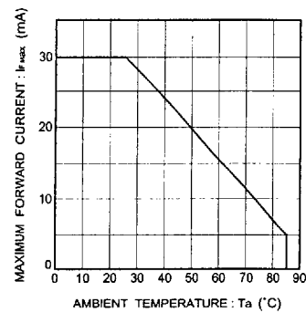
Fig. 7 Maximum forward current vs. ambient temperature
