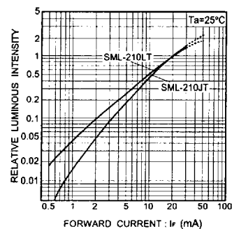
Fig. 4 Luminous intensity vs. forward current
