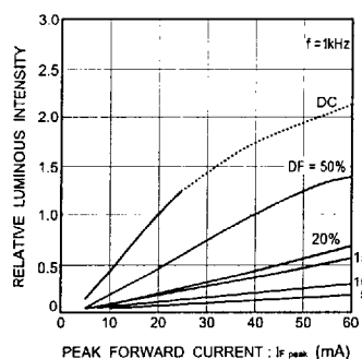
Fig. 12 Luminous intensity vs. peak forward current
