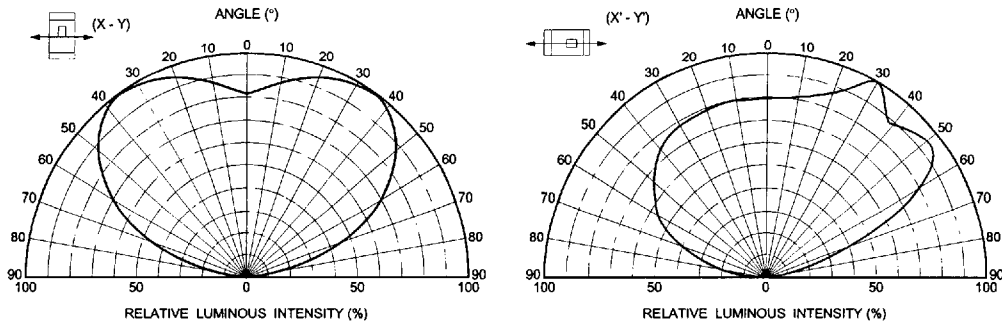
Fig.1 Directional pattern
