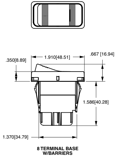
CONTURA X STYLE SHOWN WITH RAISED BRACKET
