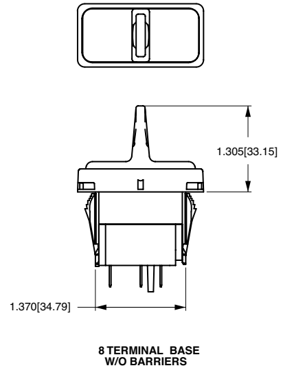
CONTURA XII STYLE SHOWN WITH PADDLE ACTUATOR
