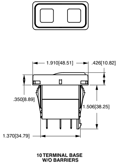
CONTURA XI STYLE SHOWN WITH RAISED BRACKET AND TWO SQUARE LENSES
