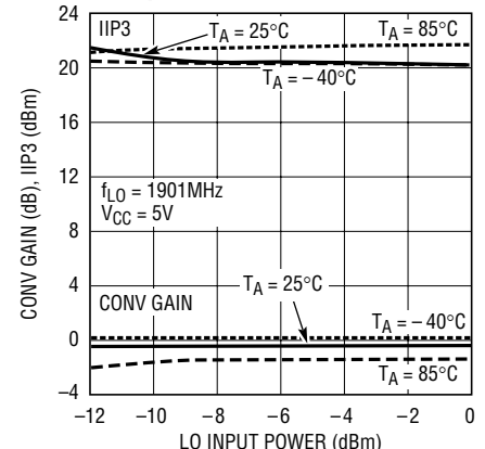
Conv Gain, IIP3 vs LO Input Power
