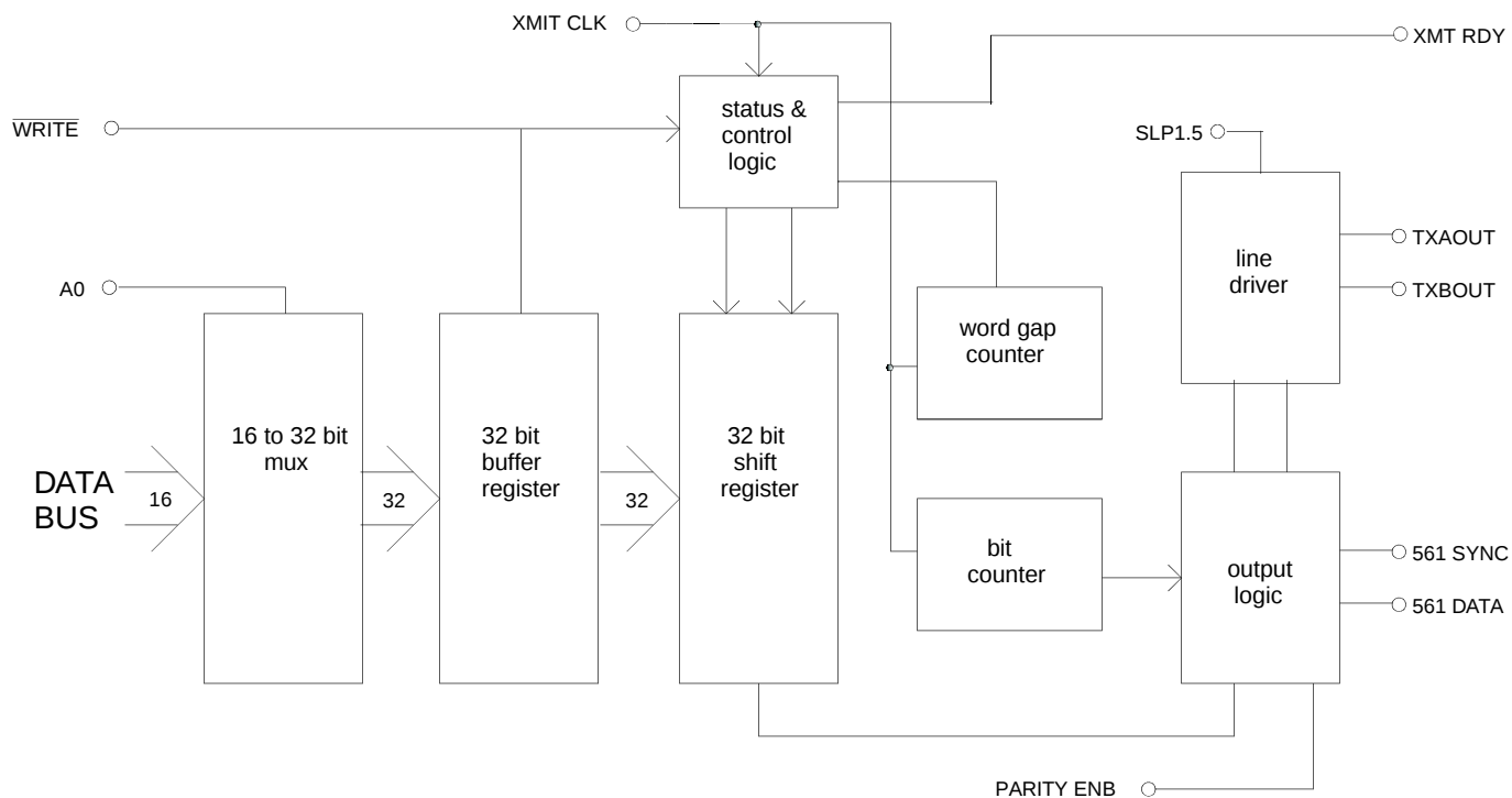
Figure 1. Block Diagram
