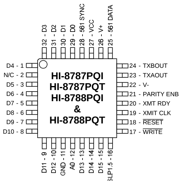
32-Pin Plastic TQFP package
