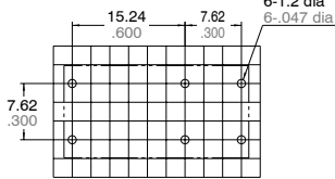
Single side stable 1 coil latching type
