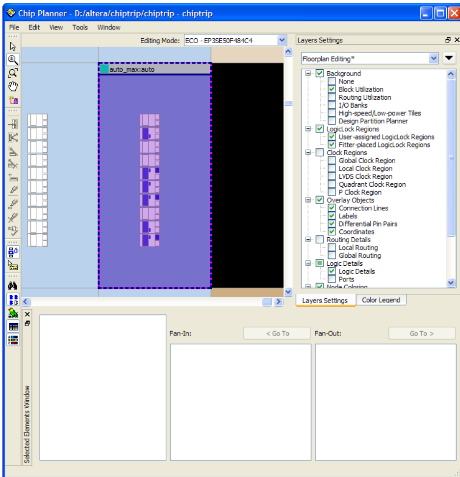
Figure 3. Chip Planner
