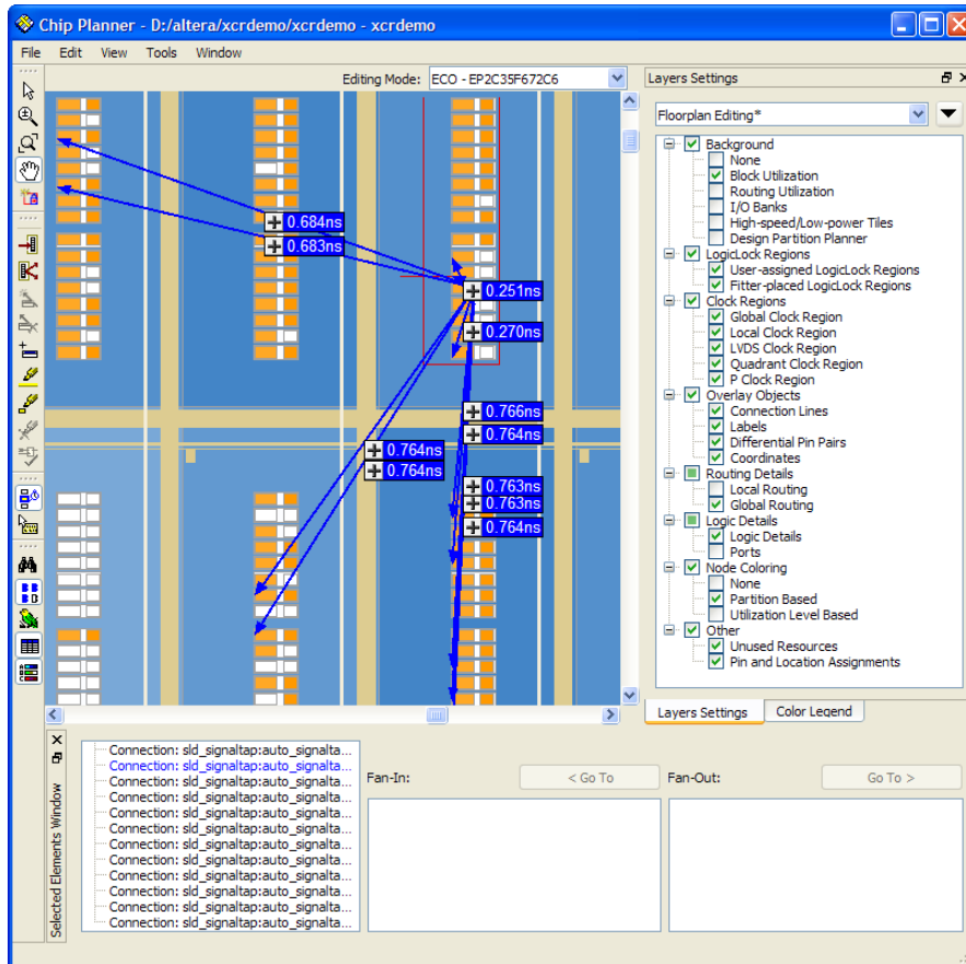
Figure 5. Chip Planner
