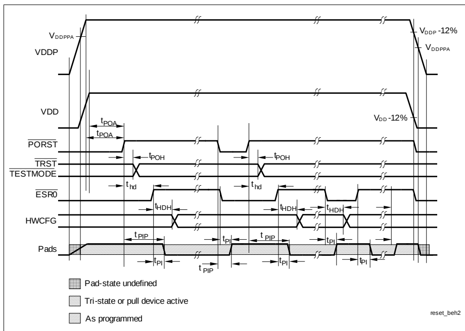
Figure 27 Power, Pad and Reset Timing
