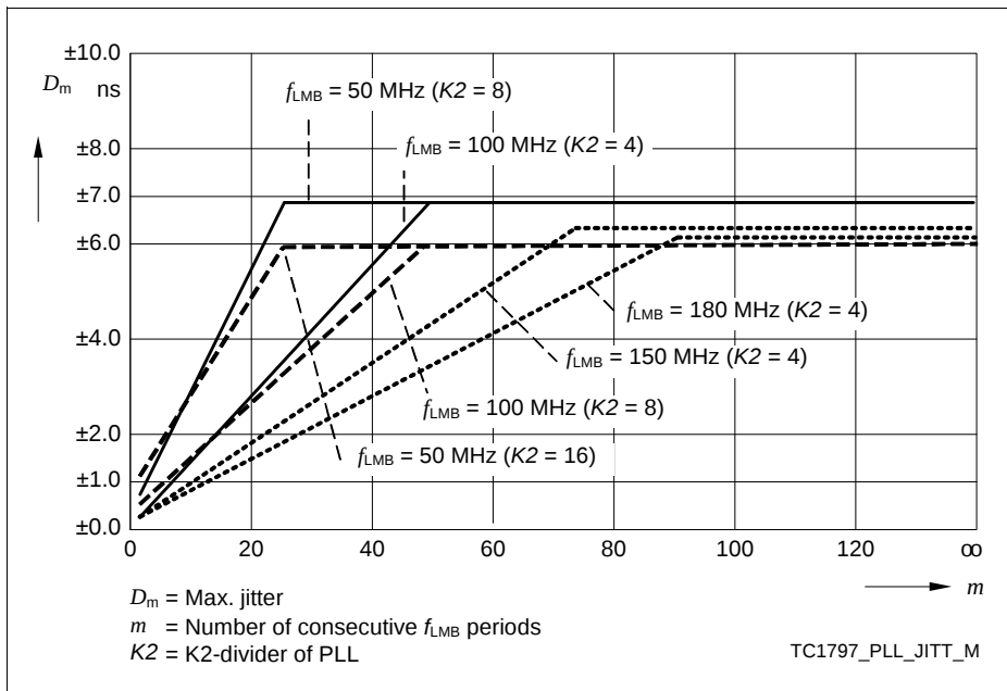
Figure 28 Approximated Maximum Accumulated PLL Jitter for Typical LMB-Bus Clock Frequencies f_{LMB}
