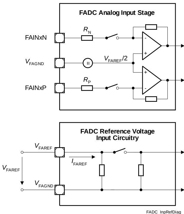
Figure 22 FADC Input Circuits
