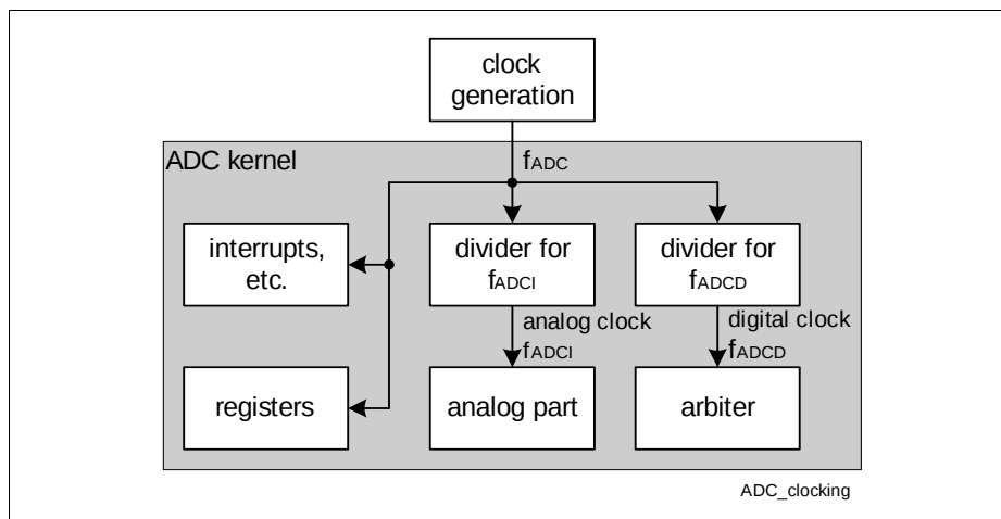
Figure 19 ADC0/ADC1 Clock Circuit
