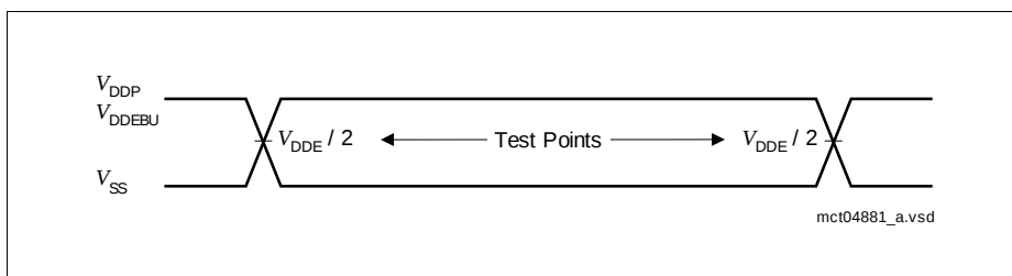
Figure 24 Testing Waveform, Output Delay
