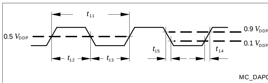
Figure 32 Test Clock Timing (DAP0)
