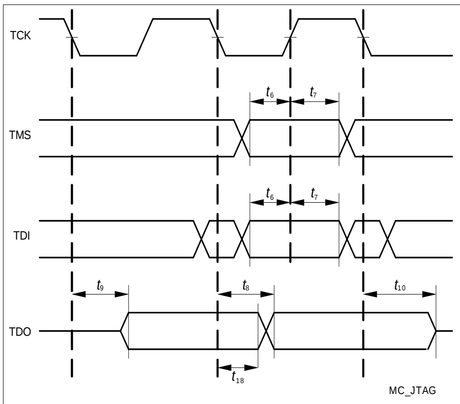
Figure 31 JTAG Timing
