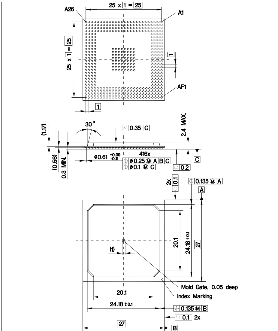
Figure 47 Package Outlines P/PG-BGA-416-27, Plastic (Green) Ball Grid Array
