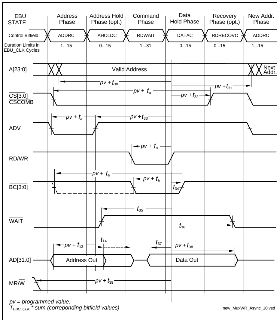
Figure 37 Multiplexed Write Access
