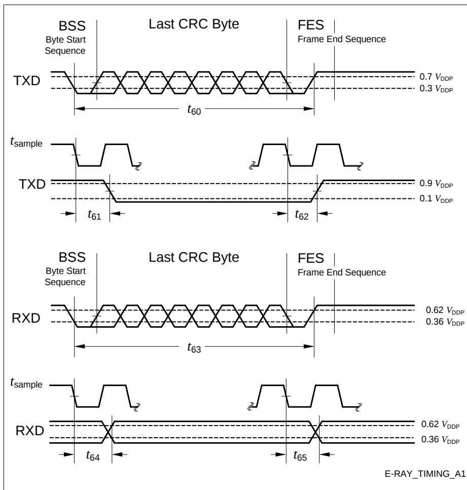
Figure 45 E-Ray Timing
