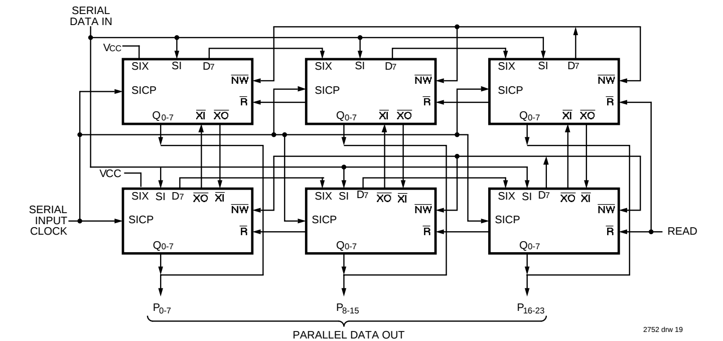
Figure 16. An 8K x 24 Serial-In, Parallel-Out FIFO Using Six IDT72142s
