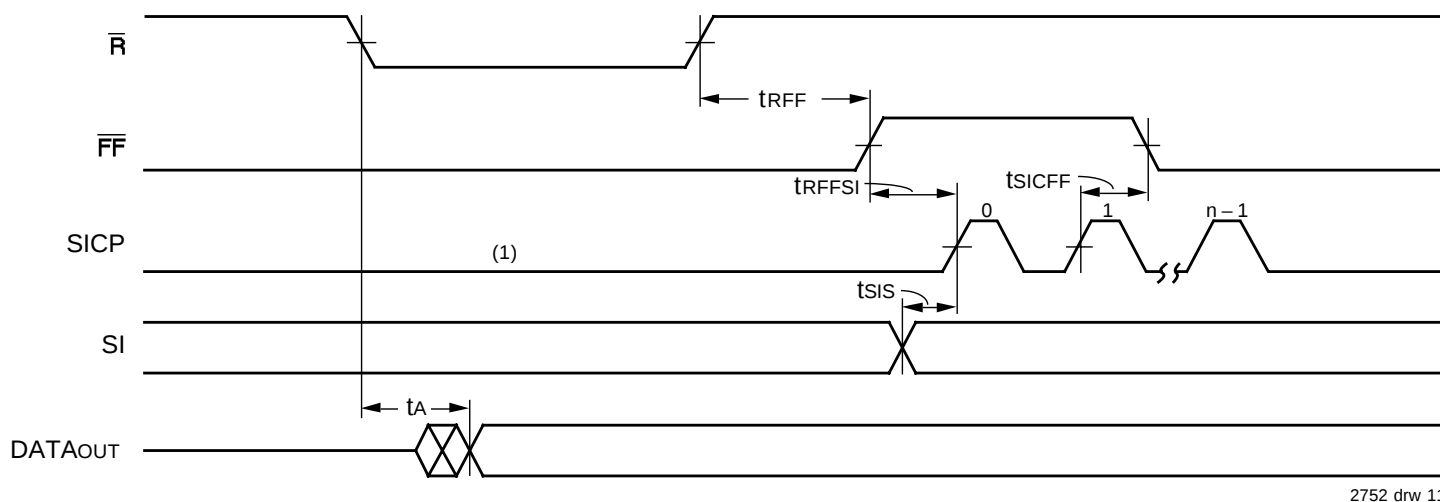
Figure 8. Full Boundary Condition Timing
