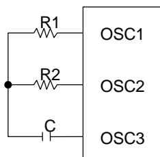
Figure 13.1 RC Oscillation
