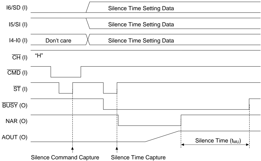
Figure 6.1 Channel 1 Silence Set Timing (Parallel Input)
