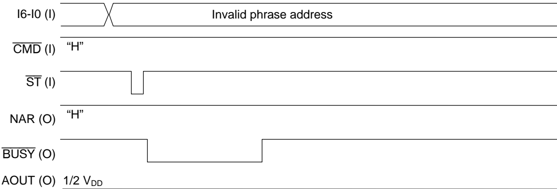
Figure 7.3 Timing when Address, Other than a Phrase, is Input when AOUT is 1/2 V_{DD}
