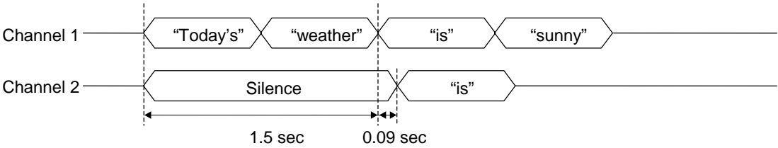
Figure 6 Playback Timing Using Table 14 Phrase Control Table
