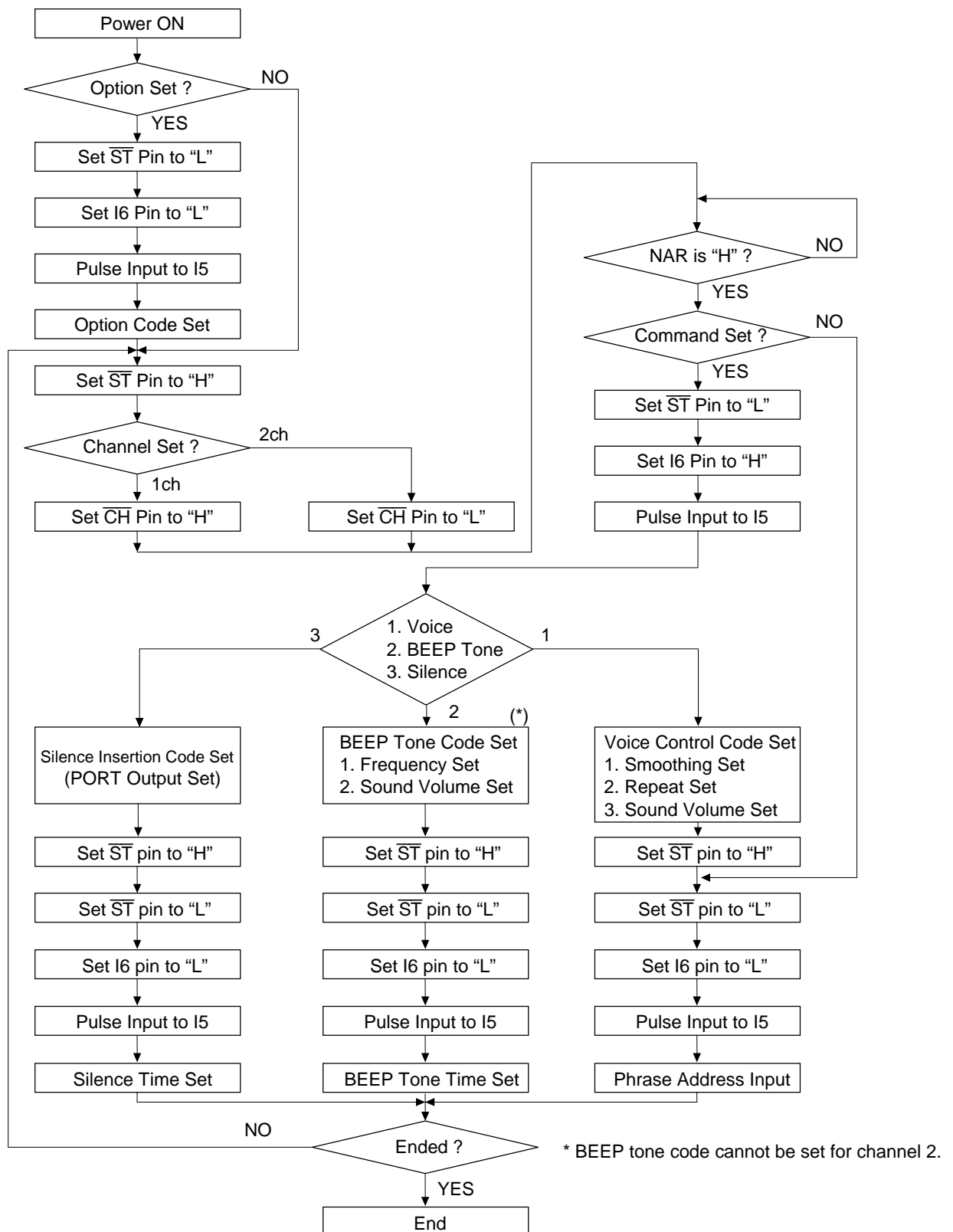
Figure 5.5 Serial Input Flowchart when External Command is Used
