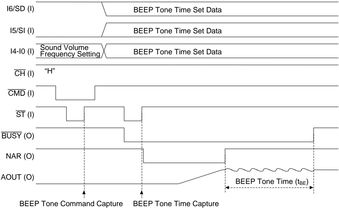
Figure 6.4 BEEP Set Timing (during Parallel Input)
