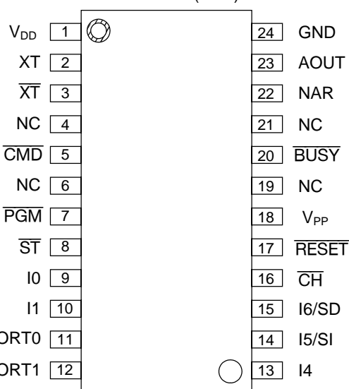
MSM66P56 (OTP)
