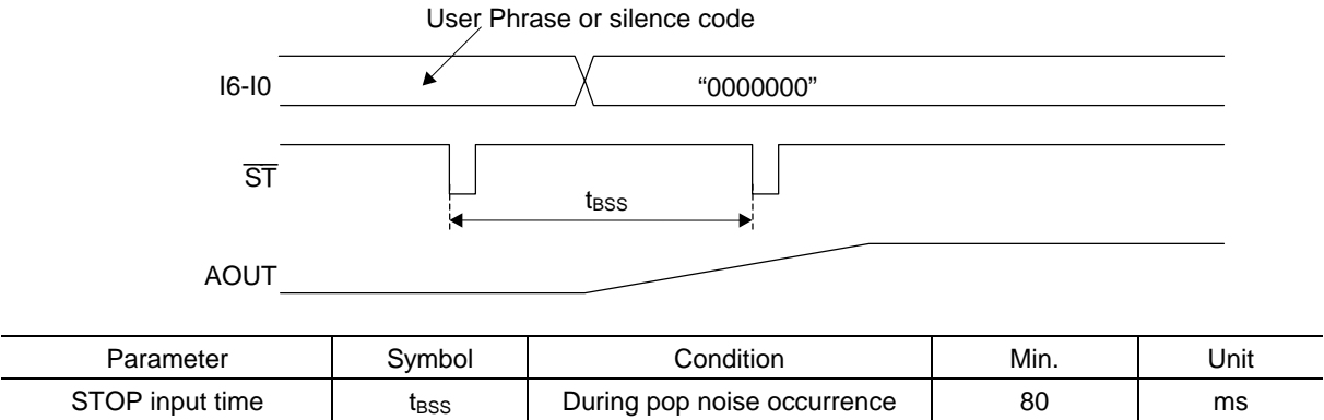
Figure 8.1 STOP Code Input Timing
