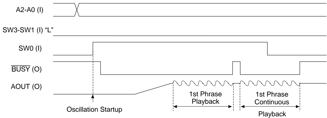
Figure 5.2 SW Input Interface - Repeated Playback Timing
