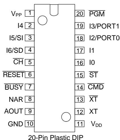
MSM66P56 (OTP)
