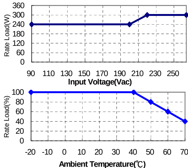
360W With Natural Convection
