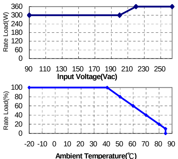
360W With Baseplate Cooled
