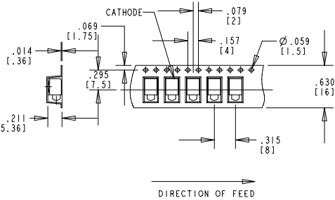
LED SCHEMATIC
