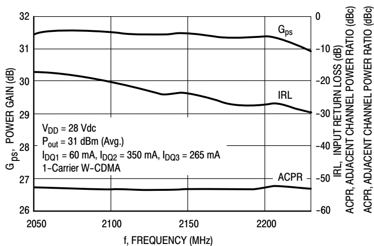
Figure 6. Single-Carrier W-CDMA Wideband Performance @ P_{out} = 31 dBm
