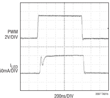
10,000:1 PWM Dimming at 100Hz
