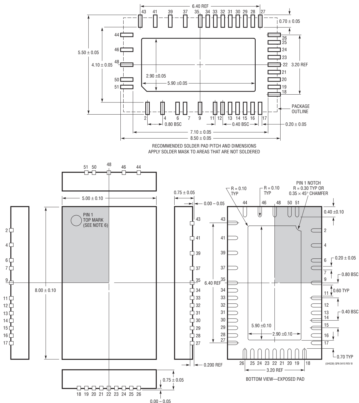
UHG Package Variation: UHG52 (39) 52-Lead Plastic QFN (5mm × 8mm) (Reference LTC DWG # 05-08-1846 Rev B)
