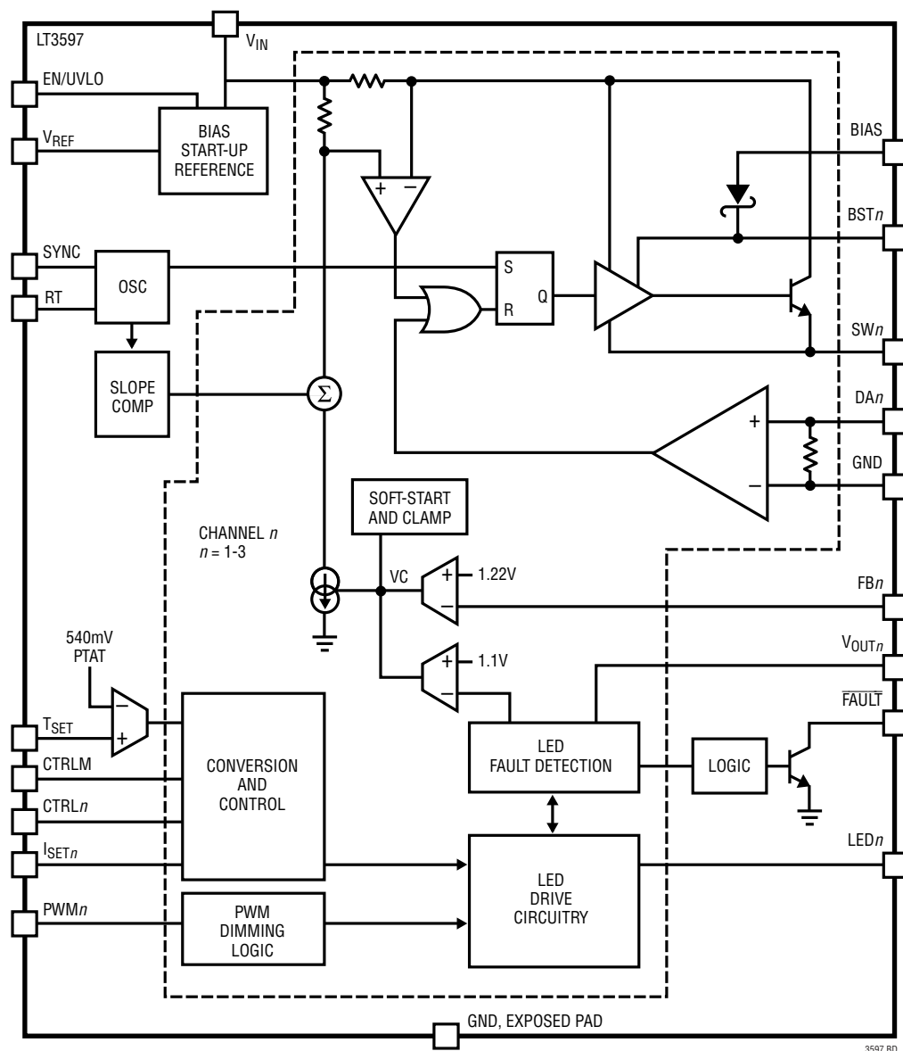
Figure 1. Block Diagram
