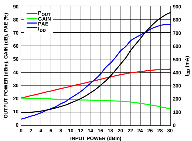
Figure 34. Output Power, Gain, PAE, and I_{DD} vs. Input Power at 0.02 GHz
