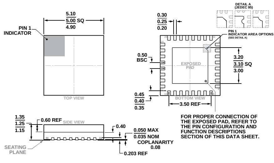
Figure 51. 32-Lead Lead Frame Chip Scale Package, Premolded Cavity [LFCSP_CAV] 5 mm x 5 mm Body and 1.25 mm Package Height (CG-32-2) Dimensions shown in millimeters
