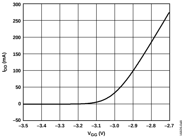
Figure 48. I_{DD} vs. V_{GG} at V_{DD} = 28\text{ V} , Representative of a Typical Device
