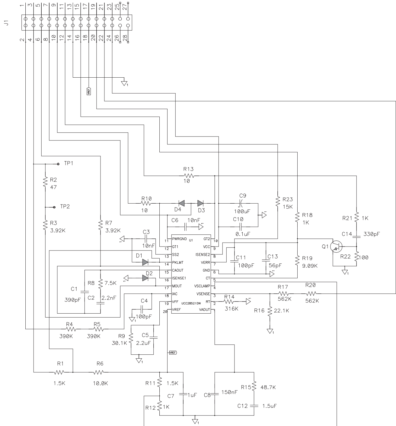
Figure 3. Daughter Board
