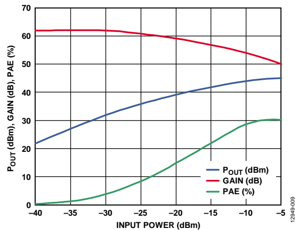
Figure 9. Power Compression at 4 GHz
