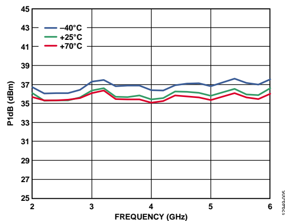
Figure 5. P1dB vs. Frequency for Various Temperatures
