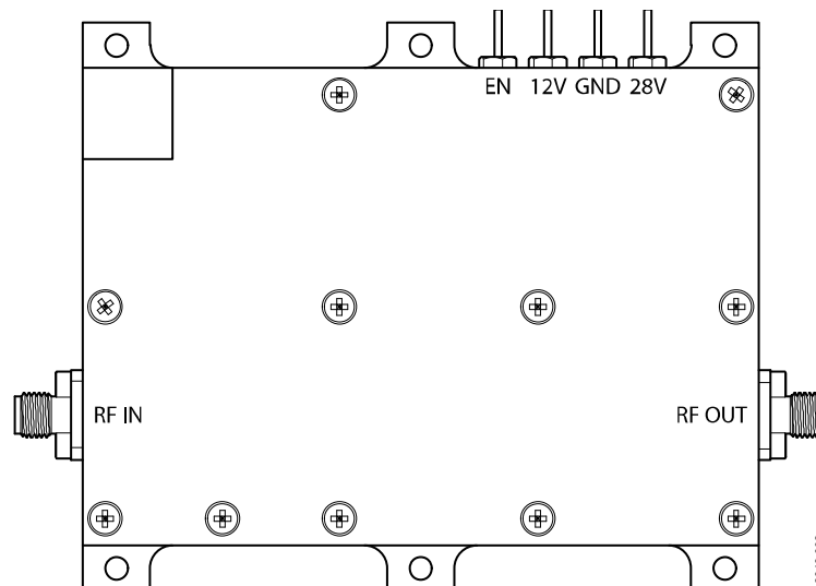
Figure 2. Pin Configuration
