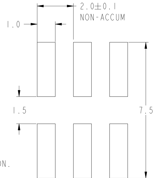
RECOMMENDED PAD LAYOUT
