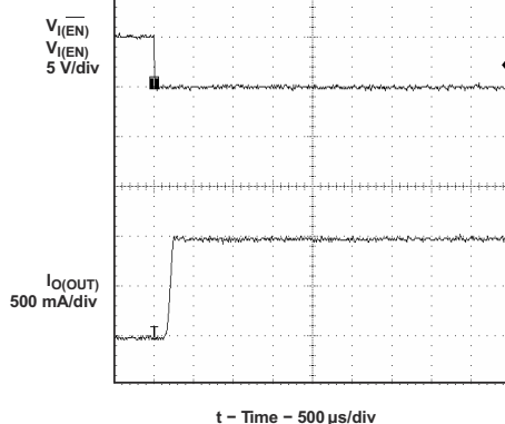
Figure 9-22. Short-Circuit Current, Device Enabled Into Short
