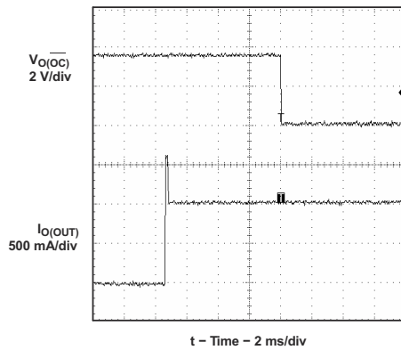
Figure 9-33. 3- \Omega Load Connected to Enabled Device
