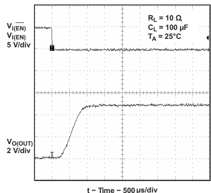
Figure 9-29. Turnon Delay and Rise Time With 100- \mu F Load
