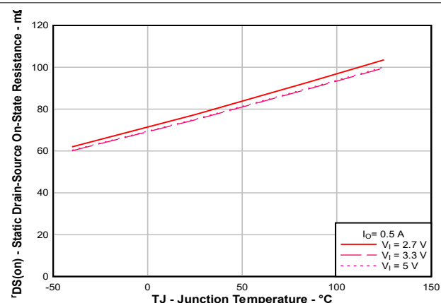
Figure 6-34. D Package Static Drain-Source on-State Resistance vs Junction Temperature
