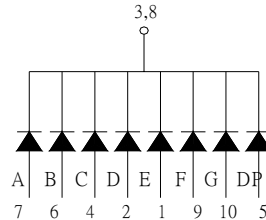
Internal Connection Diagram
