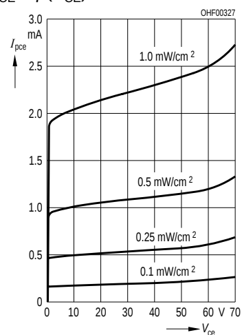
Photocurrent I_{\text{PCE}} = f(V_{\text{CE}}) SFH 3401-3
